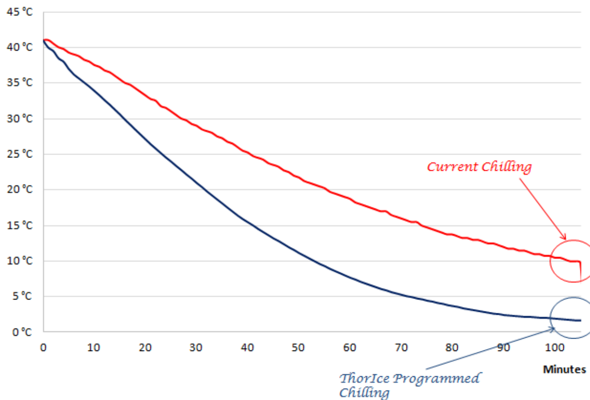
Current Chilling VS ThorIce Programmed Chilling
